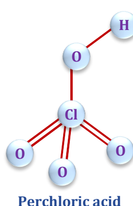
The structures of oxoacids of chlorine
