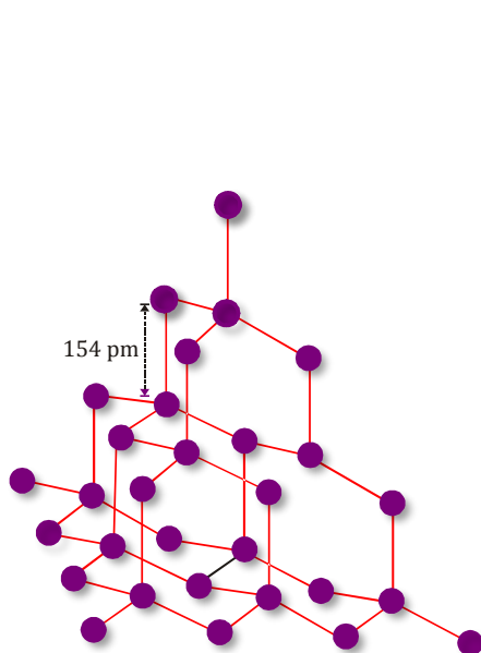
The structure of diamond
