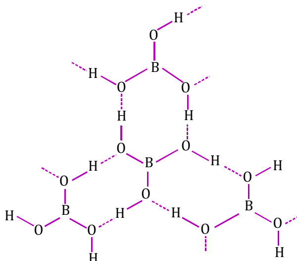
Structure of boric acid; the dotted lines represent hydrogen bonds
